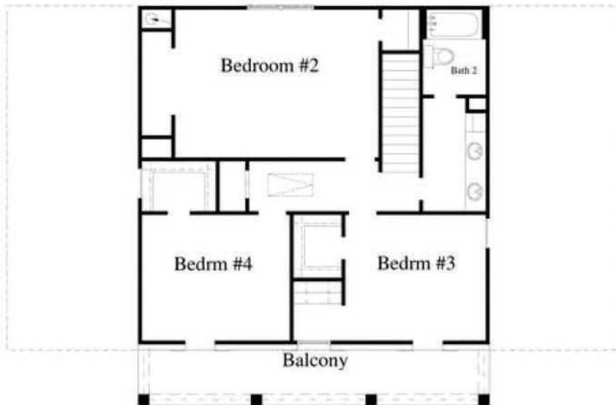
Second Floor
